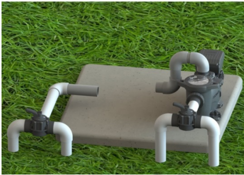
Step 1: Cut plumbing and remove StarClear Plus filter.
